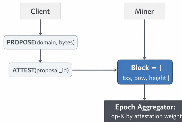
Figure 2. Transaction flow in Compute Substrate. Clients submit speculative outputs (PROPOSE) and weight them (ATTEST). Miners include transactions in proof-of-work blocks. Epoch aggregation ranks proposals deterministically without implying correctness or triggering execution.
